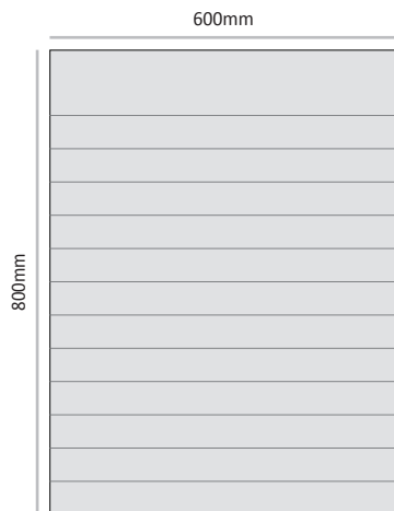
Cat. No. LEF-D-P-600-800 Unit Size WxH 600mm x 800mm
