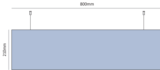
Cat. No. LEF-DS-L-210-800 Unit Size HxW 210mm x 800mm
