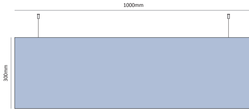
Cat. No. LEF-DS-L-300-1000 Unit Size HxW 300mm x 1000mm
